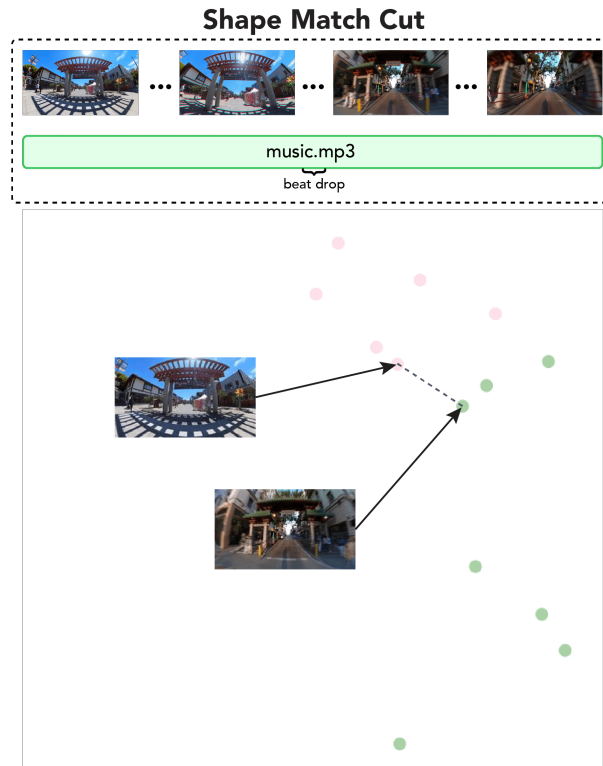
Figure 6: Under the shape lens, we can follow a path that connects across two districts to perform a shape match cut. See example result with music added.
