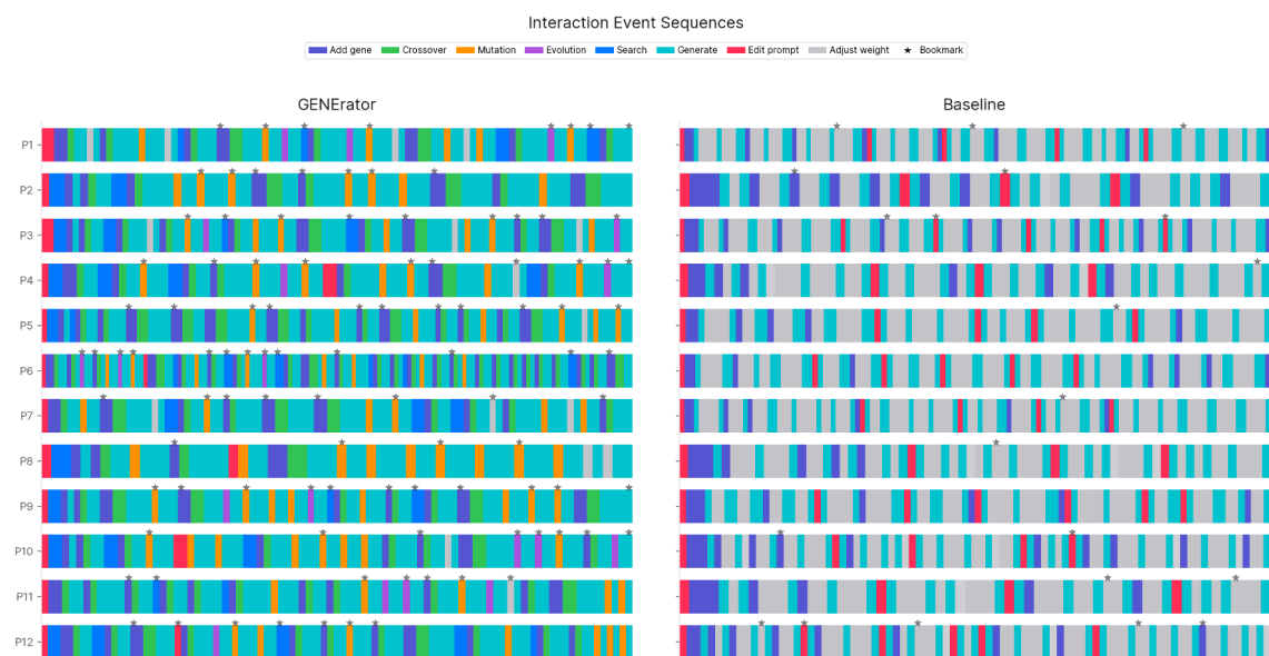
Fig. 17. Interaction event sequences for all 12 participants. Baseline (right) is dominated by trial-and-error weight adjustments and manual prompting. GENERator (left) shows a diverse mix of crossover, mutation, evolution, and semantic search operations across all participants. More designs are bookmarked (favorited) when using GENERator.
