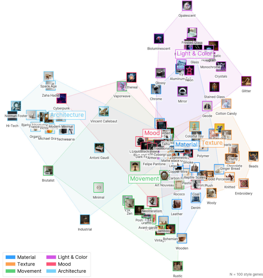
Fig. 2. The 100-gene style space projected via PCA, with convex hulls drawn around six categories of related styles. Semantically related styles cluster without explicit supervision: e.g., architectural styles (upper left), luminous effects (top), reflective materials (center), and tactile textures (right).
