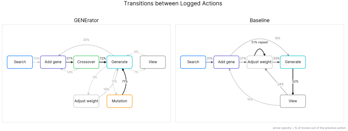
Fig. 9. Transitions between logged actions across participants. Arrows show the share of moves from one action to the next (darker is greater share). GENERator moves involve cycles of genetic operations: crossover or mutation, generate, and repeat. Baseline moves involve frequent manual slider tweaks: half of all weight adjustments were followed by another adjustment before seeing any generation.
