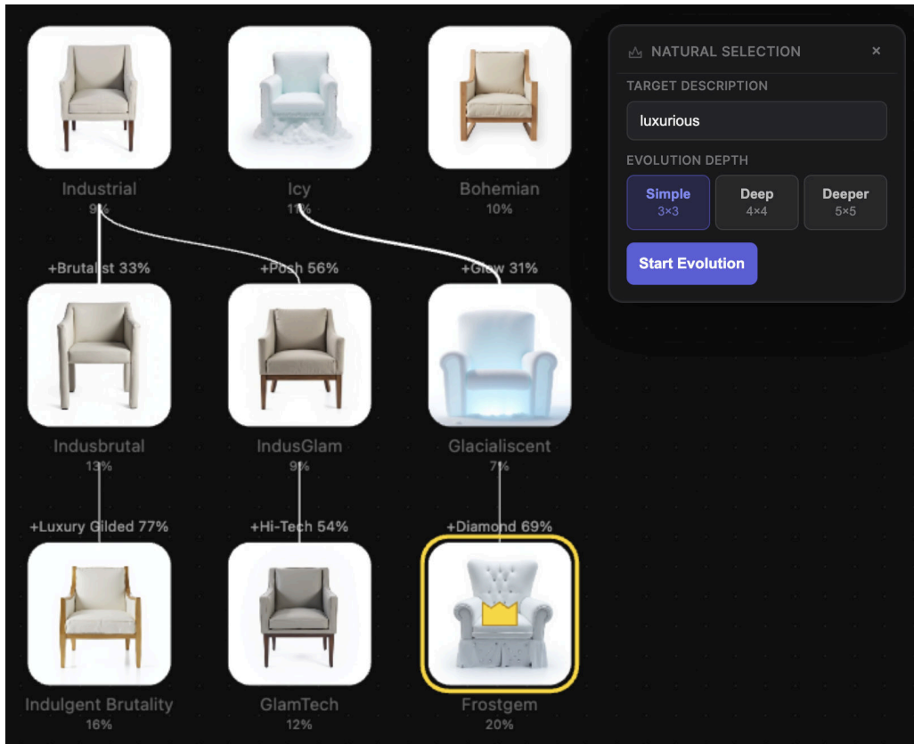
Fig. 4. Natural selection evolving a population of three styles toward “luxurious” over three generations. In each generation, the system scores every candidate among the population by similarity to the target, selects the fittest, and mutates them using semantically related genes to produce the next generation. At the final generation, the winner is selected (gold crown).
