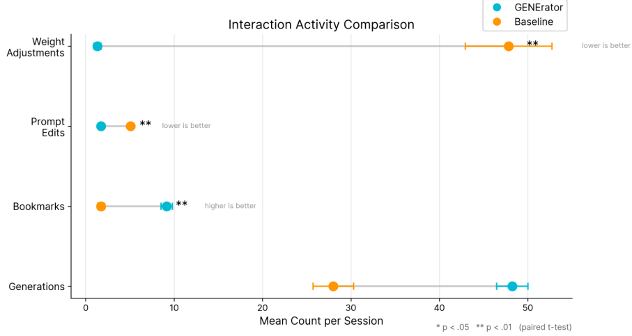
Fig. 7. Mean interaction counts per session for shared operations between GENERator and baseline (weight adjustments, prompt edits, bookmarks, generations). GENERator significantly reduced weight adjustments and prompt edits while increasing bookmarks (designs participants liked). Error bars show standard error.
