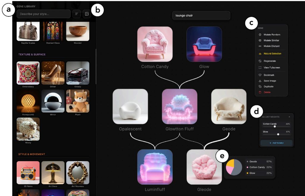
Fig. 1. The GENERator interface. (a) The designer can browse and semantically search for style genes in the gene library. (b) Genes can be dragged onto the canvas and mixed by dragging one over another. For example, crossing Cotton Candy and Glow produces the offspring Glowtton Fluff. (c) Right-clicking a gene opens a context menu of available genetic operations. Similar mutation adds Opalescent (nearby aesthetic) and distant mutation adds Geode (unrelated aesthetic). (d) The designer can adjust the weight contribution of each parent, also visualized as branch thickness in the evolution tree. (e) Hovering over a hybrid gene reveals its genetic composition.
